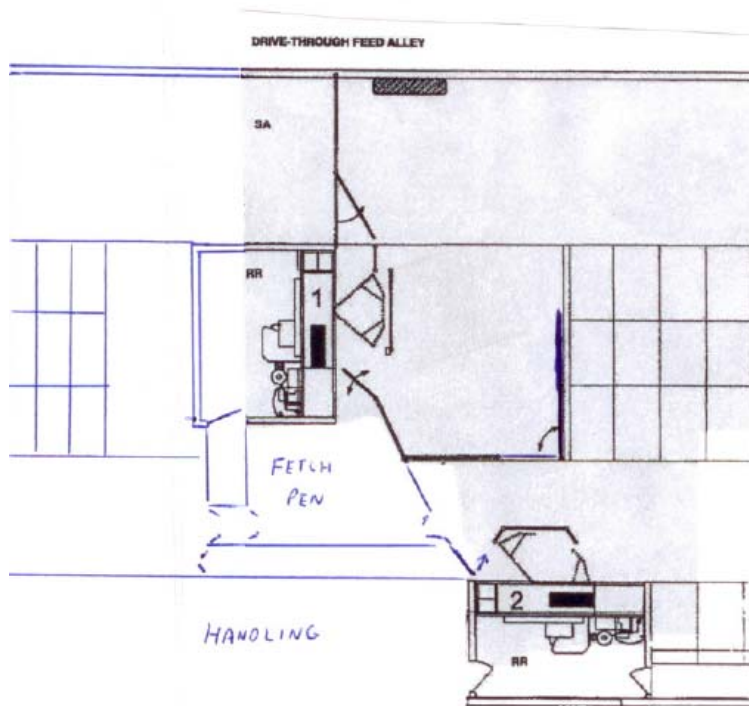
Figure 2. A 4 robot layout with handling and special needs on the left and two groups of 120 milking cows on the right.
